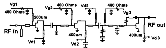
Fig. 7. LNA MMIC schematic.
