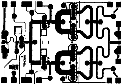
Fig. 5. PA MMIC layout.
