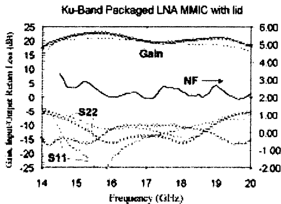
Fig. 9. Performance of Packaged LNA. Right axes is for NF curve (in dB). . MMIC chip performance is shown as dashed line.
