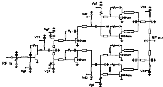
Fig. 4. PA MMIC schematic.
